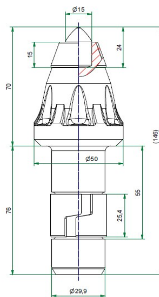
BGH09 (U84 15mm合金头)
